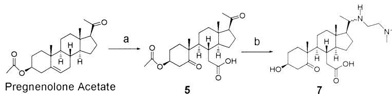
Scheme 1. Reagents: (a) O_3 , -60^\circ C , petroleum ether:ethyl acetate 1:1; piperidine; 2 M HCl, 60%; (b) N,N -dimethylethylenediamine, CH_3OH:THF , NaB(CN)H_3 , 25%.
