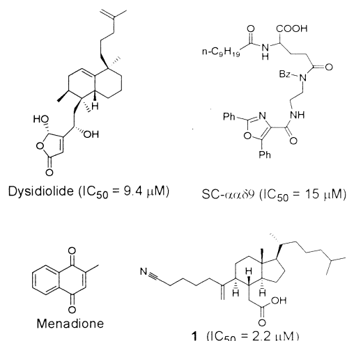
Figure 1. Chemical structures for dysidiolide, SC- \alpha\alpha\delta , menadione, and compound 1 .
