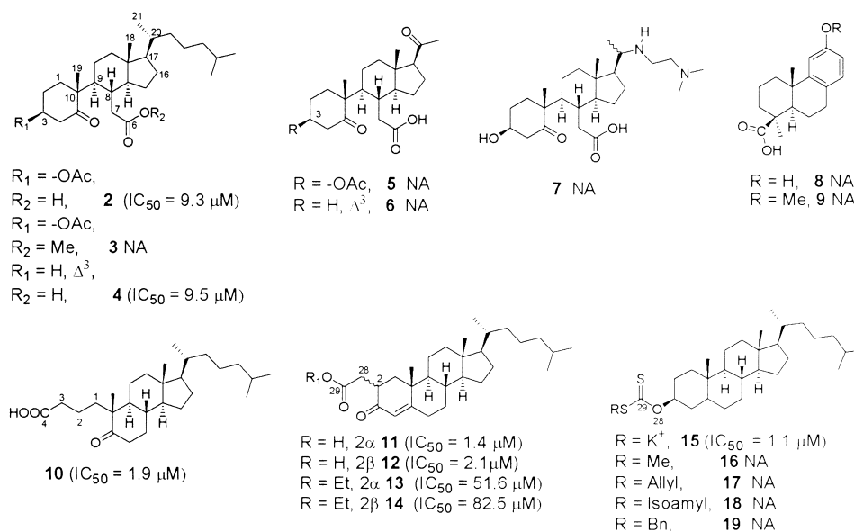
Chart 1. \text{IC}_{50} values were determined from at least two independent determinations, each run in triplicate, where the variation from the mean is \pm 20\% or less. NA stands for \text{IC}_{50} value larger than 100 \mu\text{M} . ND stands for not determined.
