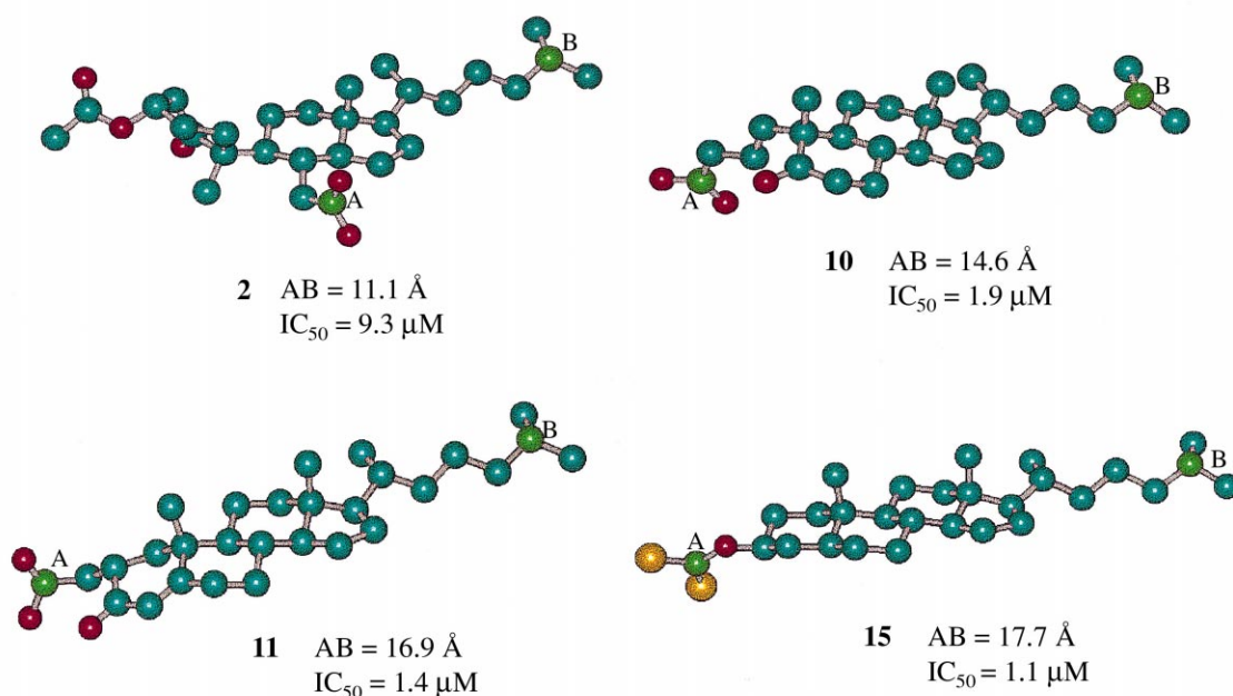
Figure 2. Calculated lowest-energy conformations for compounds 2 , 10 , 11 and 15 .
