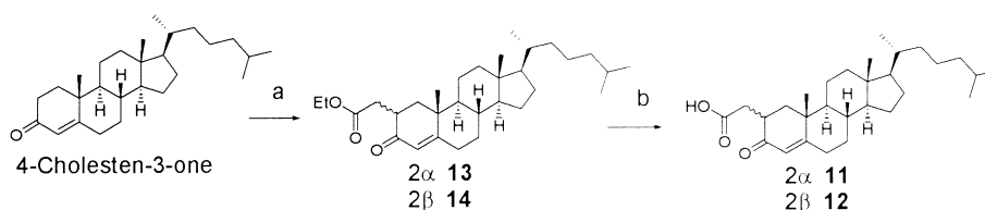
Scheme 2. Reagents: (a) LDA, THF; ethyl bromoacetate; 93%; (b) KOH, H_2O:THF ; 64%.
