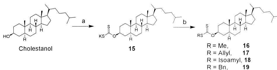
Scheme 3. Reagents: (a) K, (\text{CH}_3\text{OCH}_2\text{CH}_2)_2\text{O} , \text{CS}_2 , 85%; (b) RX, DMSO (X = Cl, Br, or I), 80–85%.
